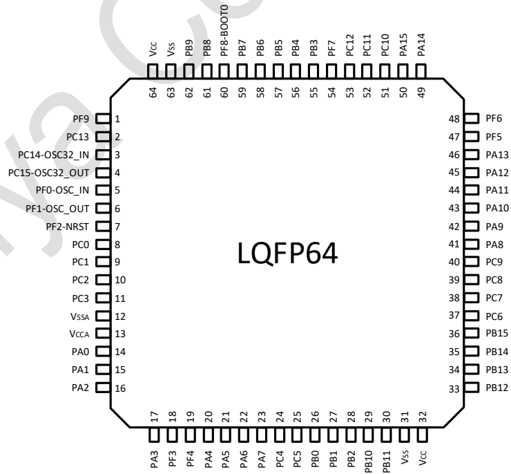
图 3-2 LQFP64 PY32F040R2xT6 Pinout2 (Top view)
