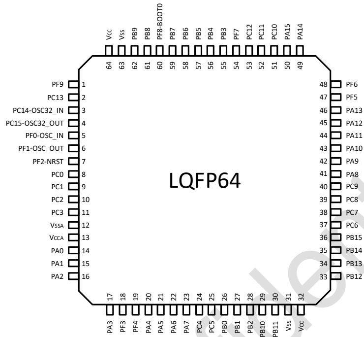
图 3-1 LQFP64 PY32F040R1xT6 Pinout1 (Top view)
